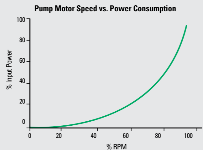
This graph shows the huge increase in energy consumption as pump speed increases. Slow down the pump and you cut energy costs dramatically.
