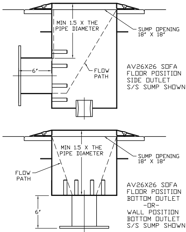
Sketch of SOFA Side View
