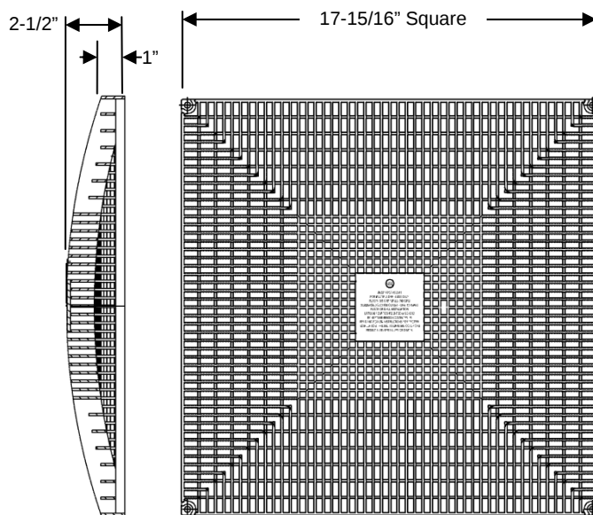
GRATING DETAIL
