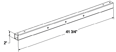
2X (P) FRAME END TUBE 60.1300.003
