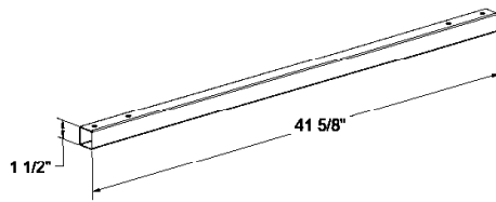
2X (N) FRAME SIDE TUBE 60.1225.001
