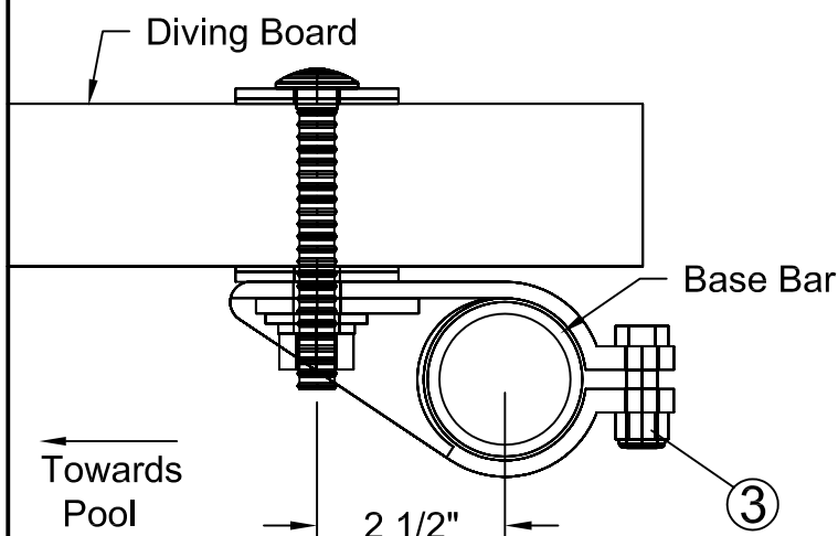
Side View of Part # 18403
