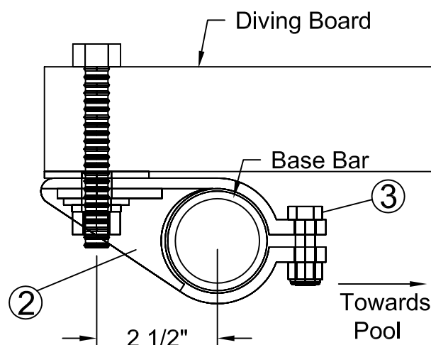
Side View of Part # 18401 and Part # 18402
