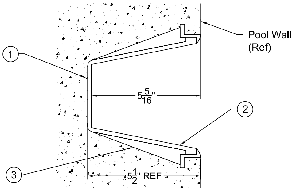
SECTION X-X
