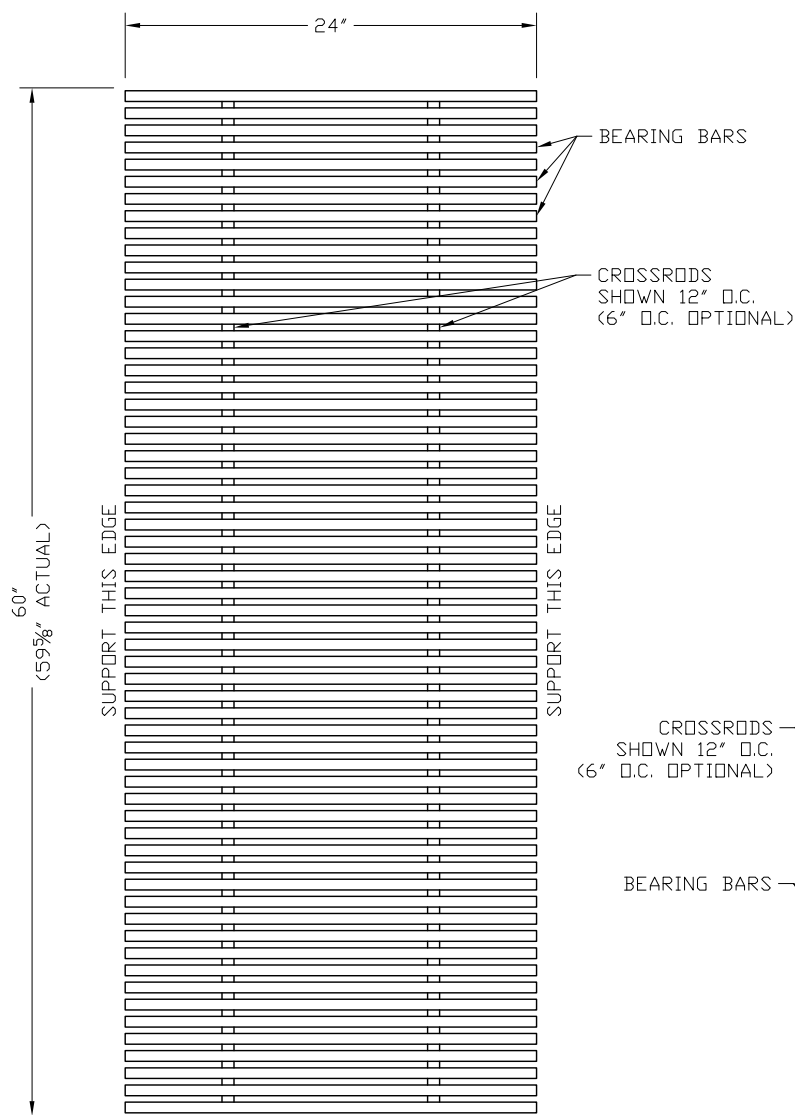
60" WIDE X 24" B.B.
