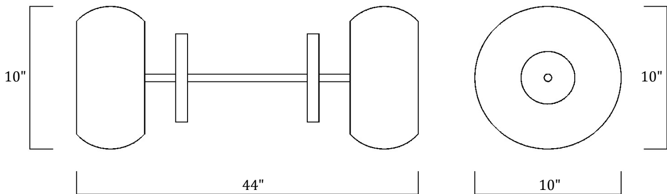
Front View
