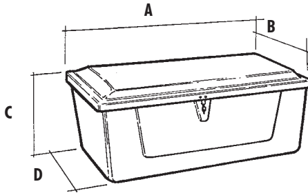
Seat-N-Stor Dimensions
